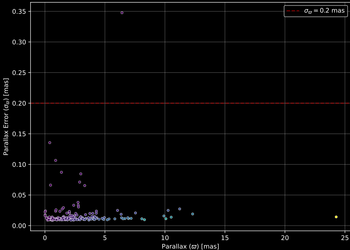
APOGEE DR17 Field: [271-31-O_TESS] Parallax Quality (n= 188)
