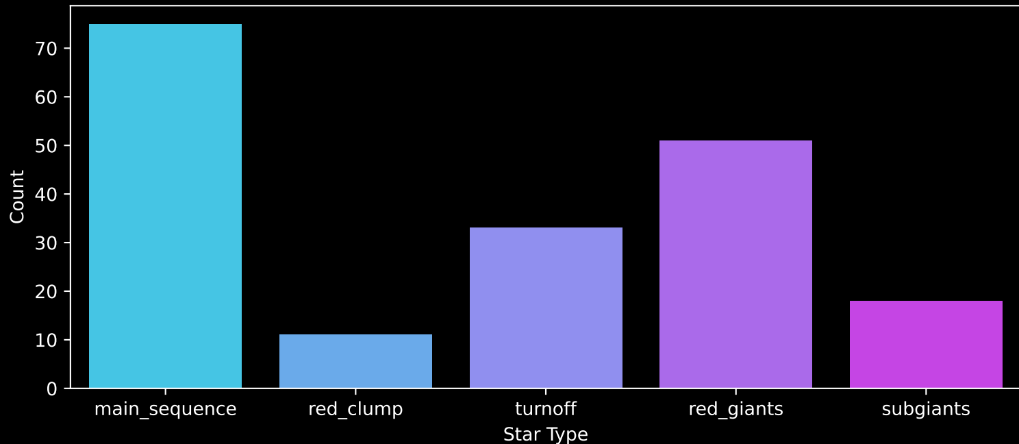
APOGEE DR17 Field: [271-31-O_TESS] Count plot of Star Type
