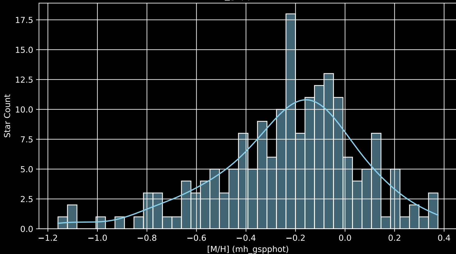
APOGEE DR17 Field: [271-31-O_TESS [M/H] (mh_gspphot) (n= 185)
