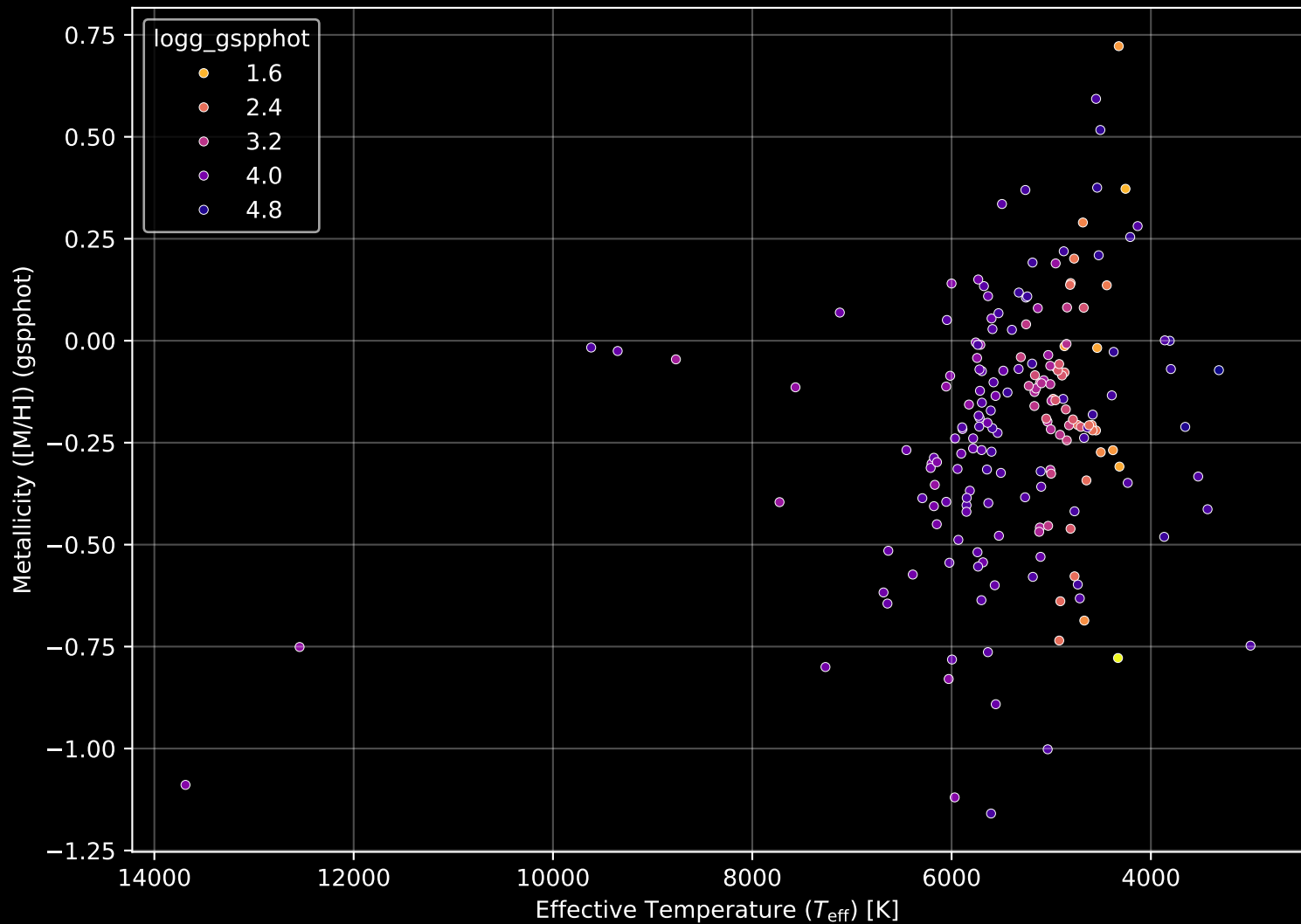
APOGEE DR17 Field: [271-31-O_TESS] Stellar Population Parameters (n= 188)
