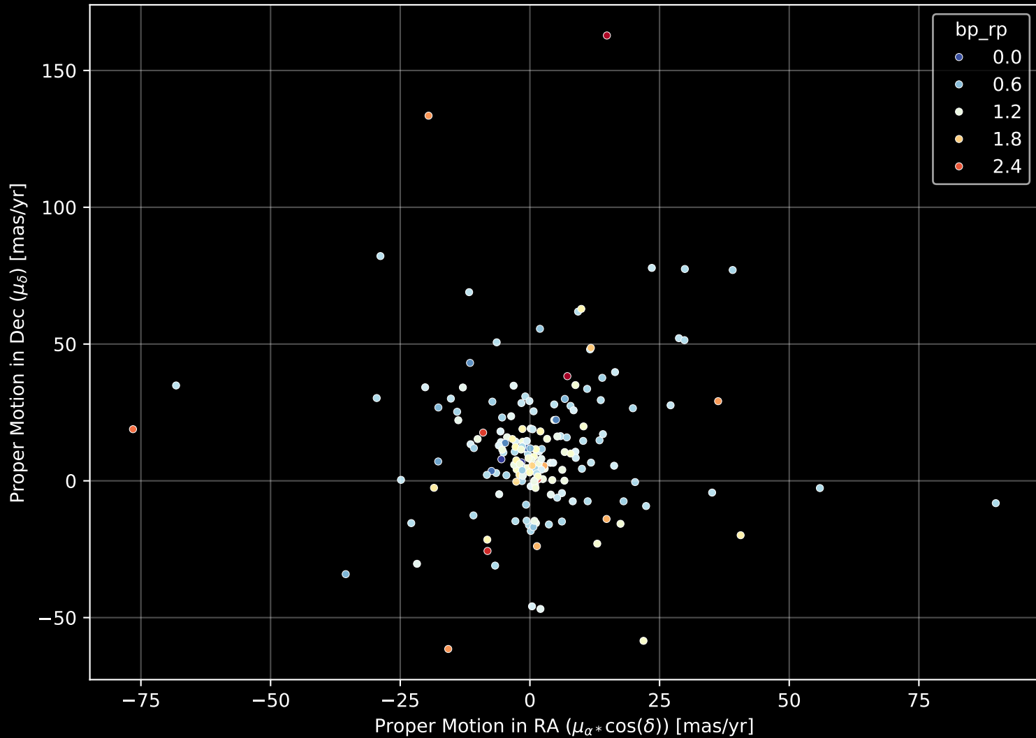
APOGEE DR17 Field: [271-31-O_TESS] Proper Motion Diagram (n= 188)
