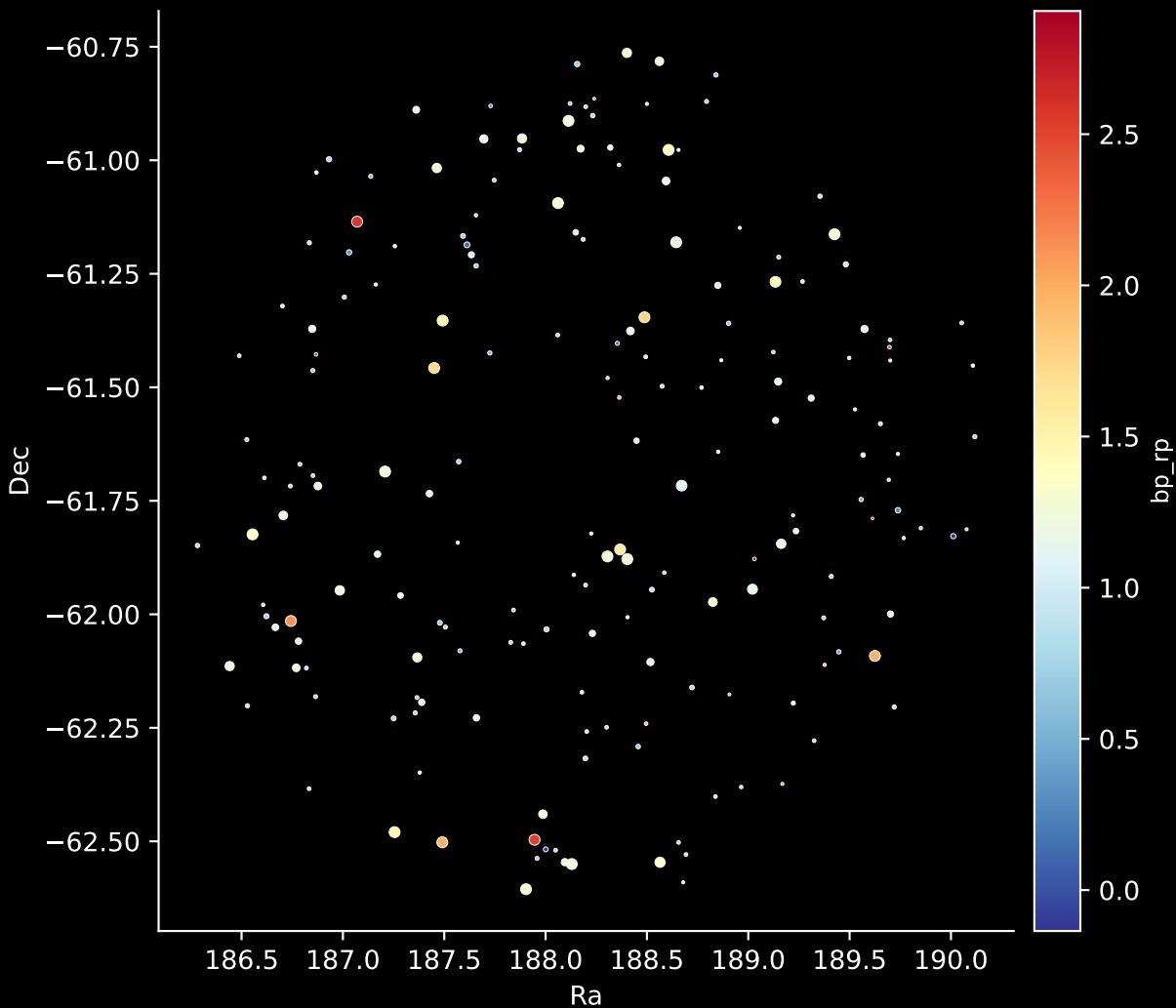
APOGEE DR17 Field: [271-31-O_TESS] Stars: 188
