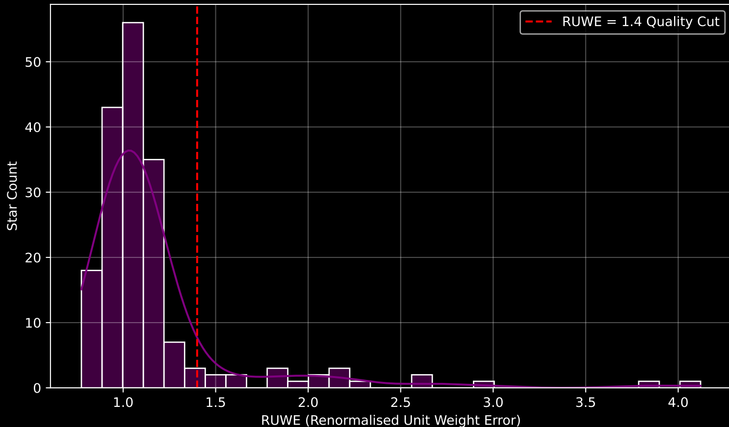
GAPOGEE DR17 Field [271-31-O_TESS] RUWE Distribution (n= 181)
